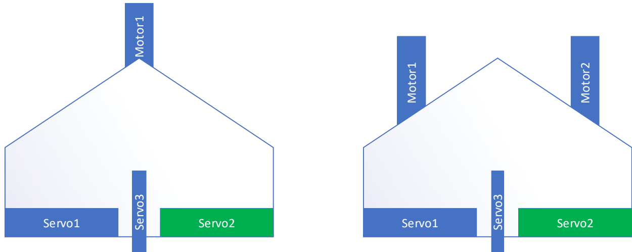
Figure 18 – MIXER_FLYING_WING
