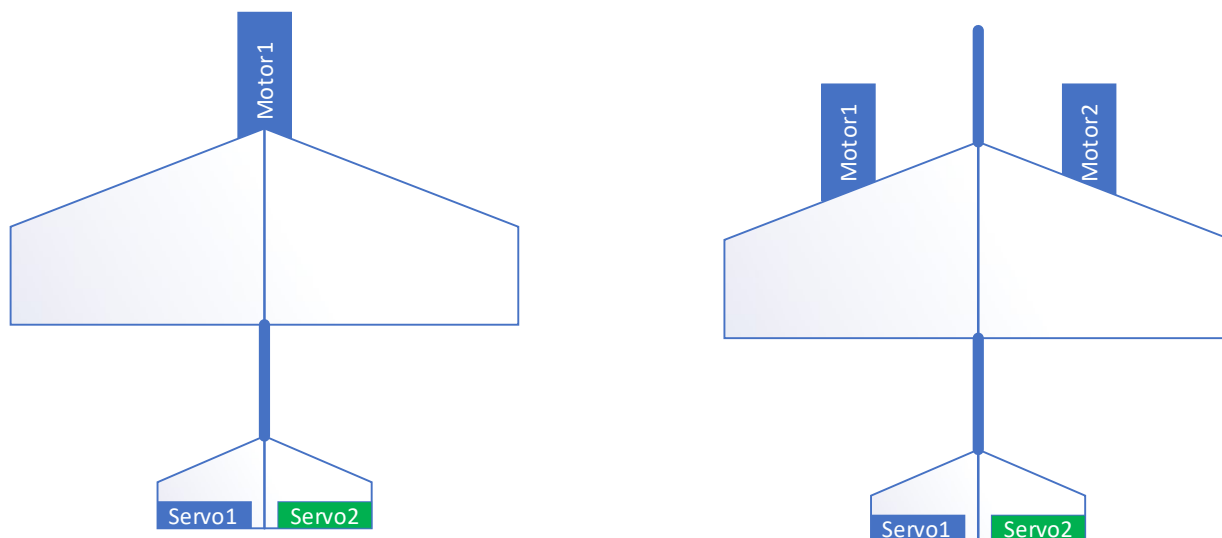
Figure 17 - PLANE_V_TAIL
