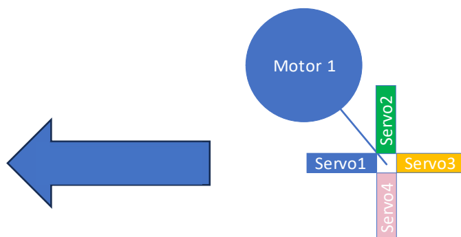
Figure 23 – SINGLE_COPTER
